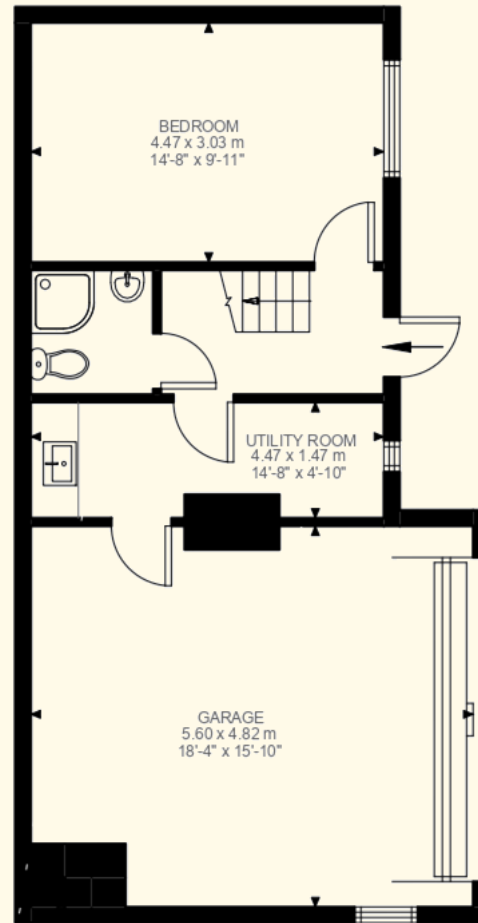
Ground Floor 304 ft 2
